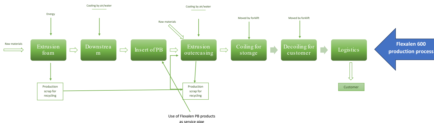
Figure 3 : Manufacturing process
