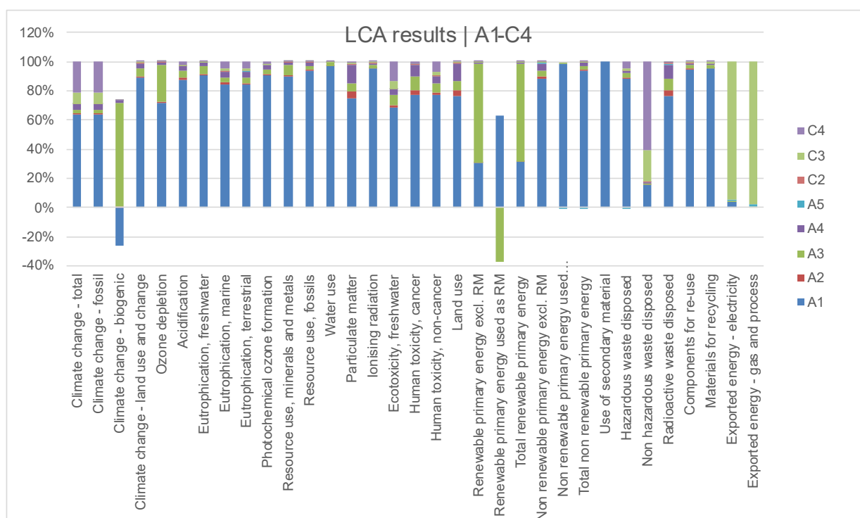
Figure 4 : LCA results for modules A1 to C4 (European EN15804+A2 indicators)
